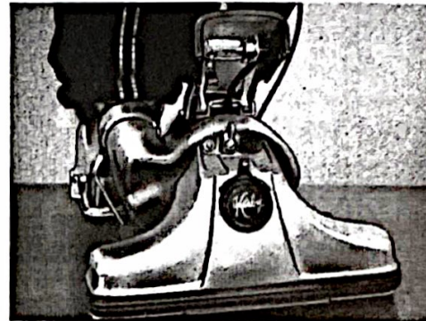
← FIGURE 3 Position of belt lifter when belt is driving brush.
